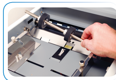
Removable Feed Wheels
